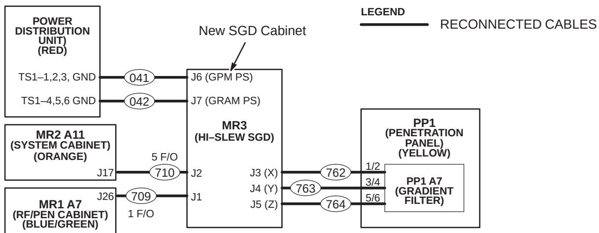
SIGNA HORIZON™ CABLES AFTER UPGRADING TO 8.x EchoSpeed with SGD ILLUSTRATION 2-6
