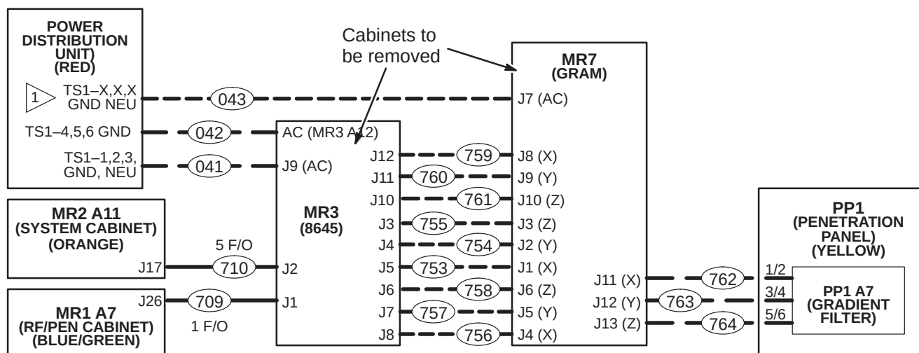
AFFECTED SIGNA HORIZON™ CABLES WHEN UPGRADING FROM 1.5T EchoSpeed TO EchoSpeed with SGD ILLUSTRATION 2-5
